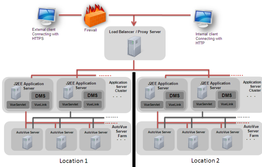
Figure 4–1 Standalone/Non-Integrated Deployment
