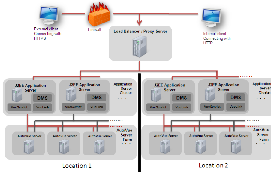
Figure 4–8 Disaster Recovery
