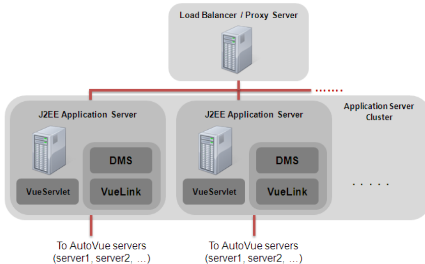
Figure 4–4 VueServlet Cluster
