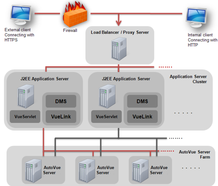
Figure 4–7 Failover Deployment
